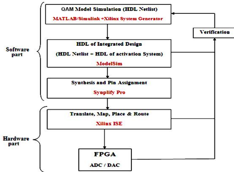
Figure (3): Proposed Simulation and implementation flow
