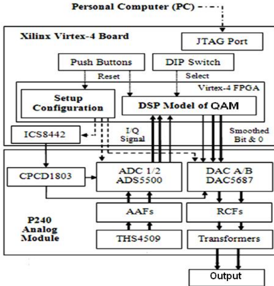
Figure (9): Hardware Implementation of FPGA and P240.
