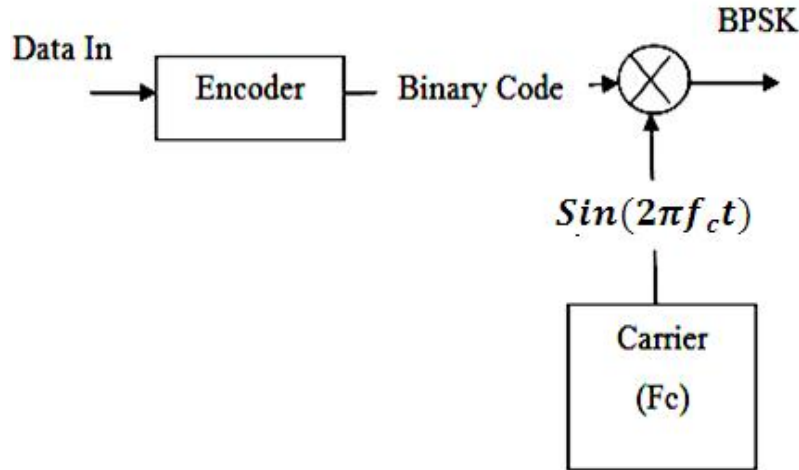
Figure (2): Block diagram of BPSK modulator design
