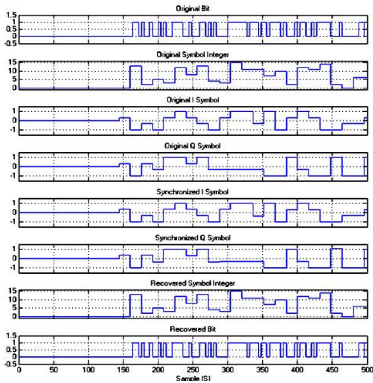
Figure (5): Simulation Results of QAM
