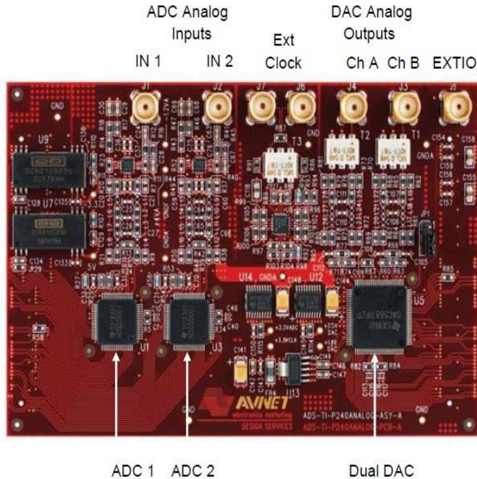
Figure (8): Avnet Electronics Marketing P240 Analog Module [23] .
