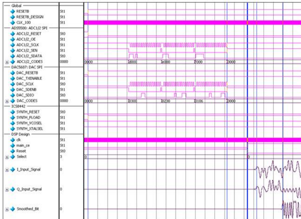
Figure (6): HDL simulation result of QAM Netlist
