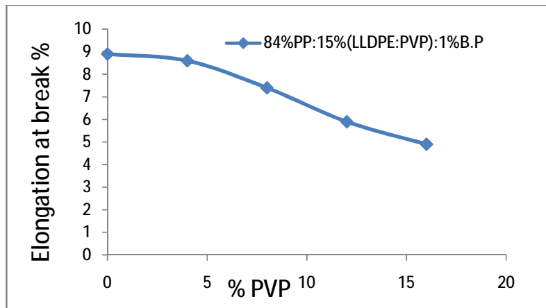
Figure.(6 b) Elongation of [84%PP:15%((100-X)%LLDPE:X%PVP):1%B.P] as a function of PVP content in the composites.
