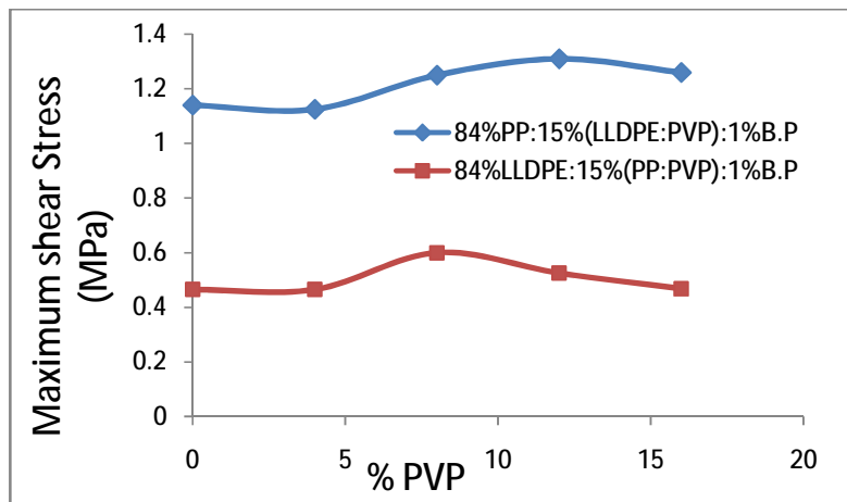
Figure. (9) Maximum shear stress of [84%LLDPE:15%((100-X)%PP:X%PVP):1%B.P] and [84%PP:15%((100-X)%LLDPE:X%PVP):1%B.P] as a function of PVP in the composites.
