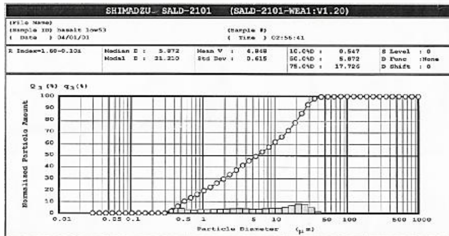
Figure. (1) Shows particle size analysis of basalt.
