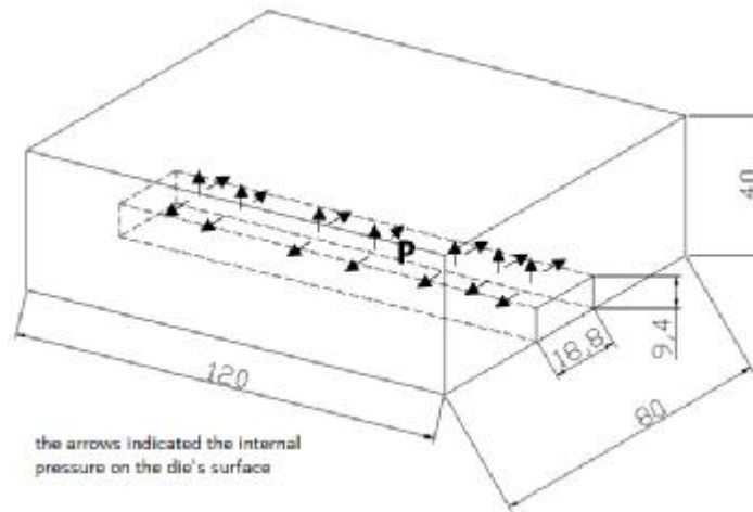
Figure (3): The loads exert on the die.
