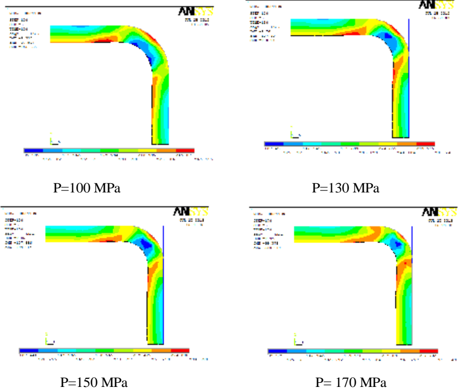
Figure (11): Effective stress distribution in the bulging tube.
