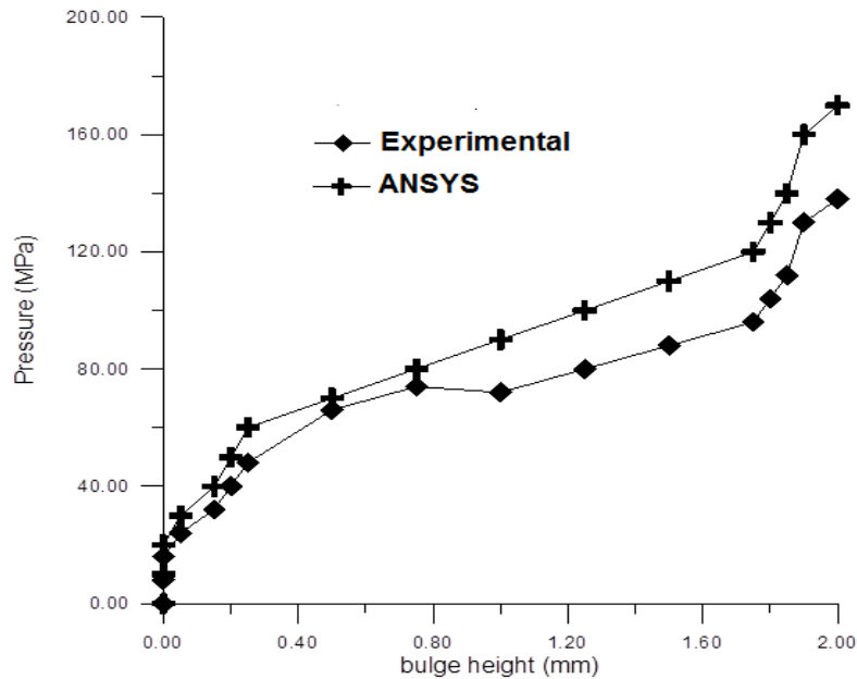
Figure (15):Relationship between internal pressure and bulge height
