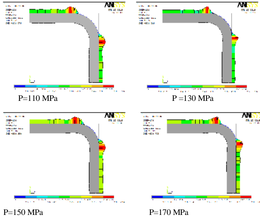
Figure (14): Show the contact pressure between the tube wall and the die
