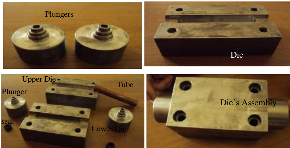
Figure(6): Hydroforming die for square cross section.
