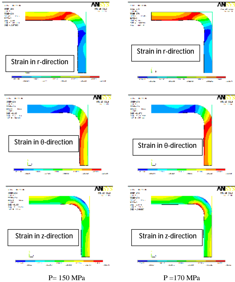
Figure (12):Strain distribution in the bulging tube in r, \theta , and z direction
