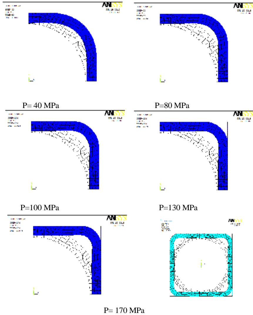
Figure (13) The deformation of the tube during bulging, show the change of the tube wall thickness.
