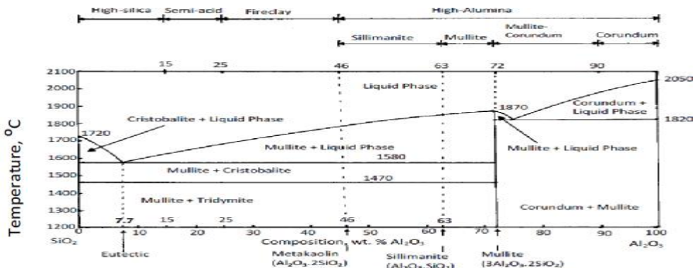
Figure (1). Phase Diagram of Al 2 O 3 and SiO 2 showing classification of aluminosilicate refractories [6].
