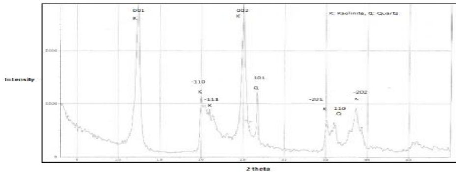
Figure (2). XRD of kaolinite raw material.
