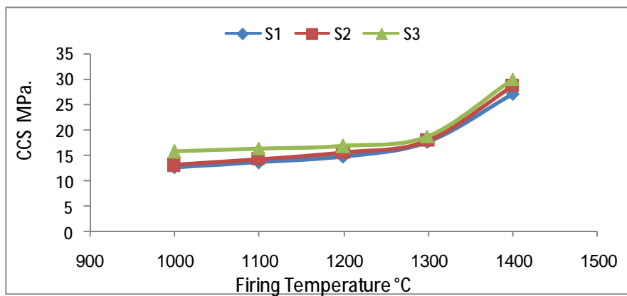
Figure (6). Relationship between CCS and firing temperature.
