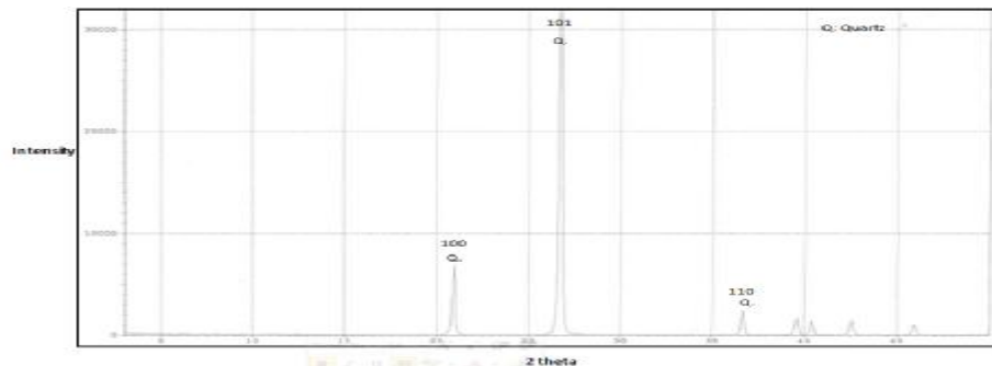
Figure (3). XRD of white sand raw material.
