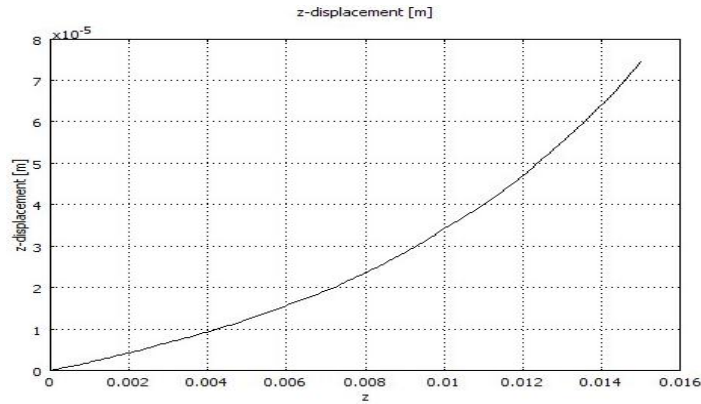
Figure (12): Z-displacement through thickness of F-FGM.
