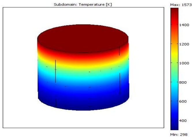
Figure (13):3-D temperature distribution of F-FGM.
