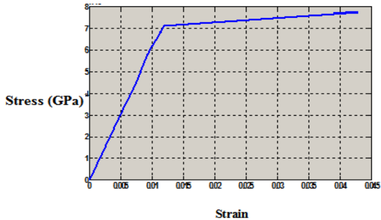
Figure (9): Stress-strain diagram of F- FGM samples.
