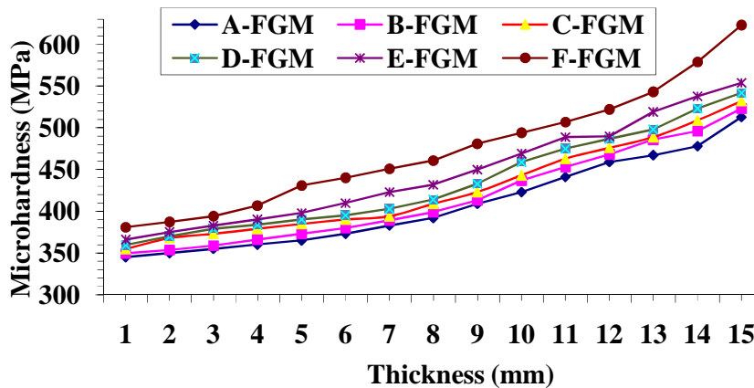
Figure (7): Microhardness variation along the FGMs thickness.
