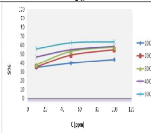
Figure (10) Sensitivity of ZnO thin film to CO 2 gas.
