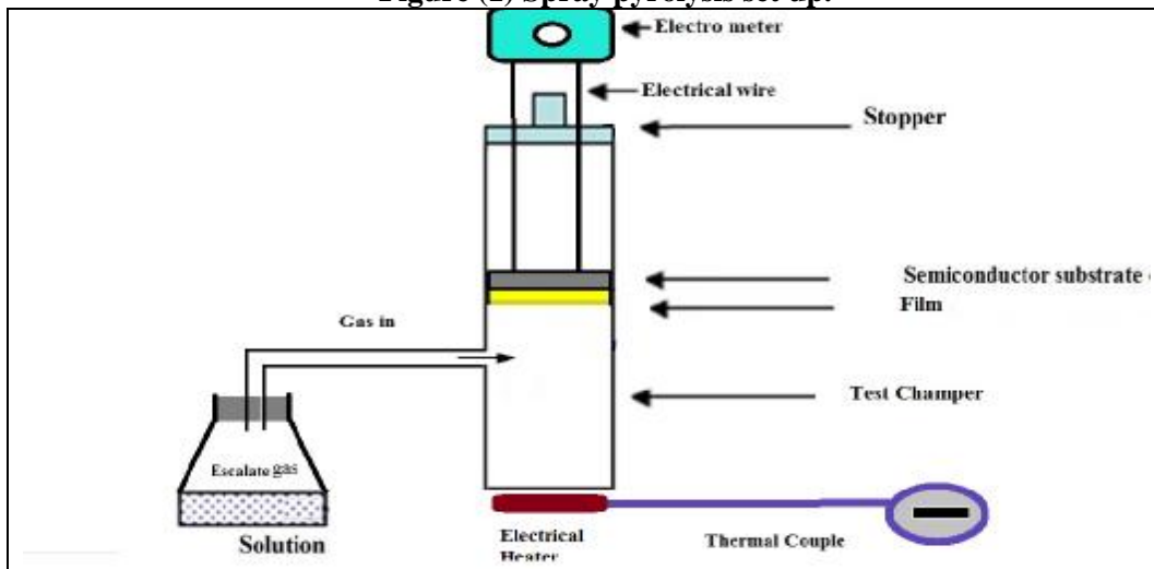
Figure (2) Detection set up.
