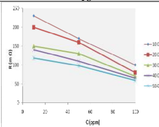
Figure (7) Resistance of ZnO thin film to NO 2 gas .
