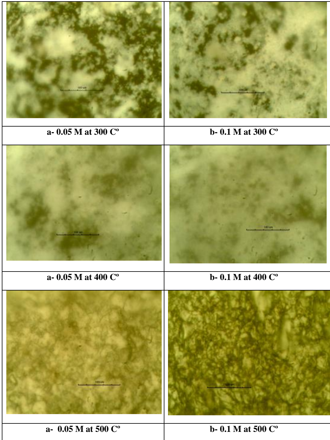
Figure (3) Optical microscope images of ZnO (X100), as a function of concentration and temperature.
