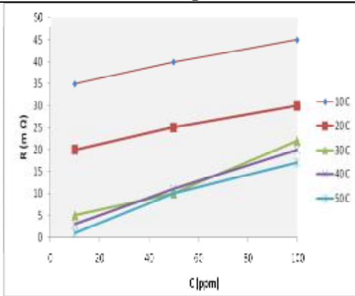
Figure (5) Resistance of ZnO thin film to H 2 S gas .
