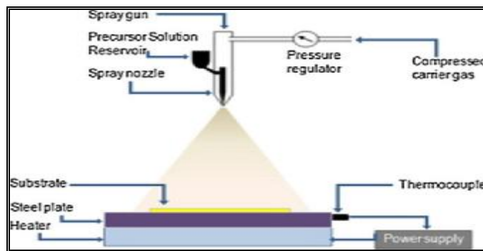
Figure (1) Spray pyrolysis set up.
