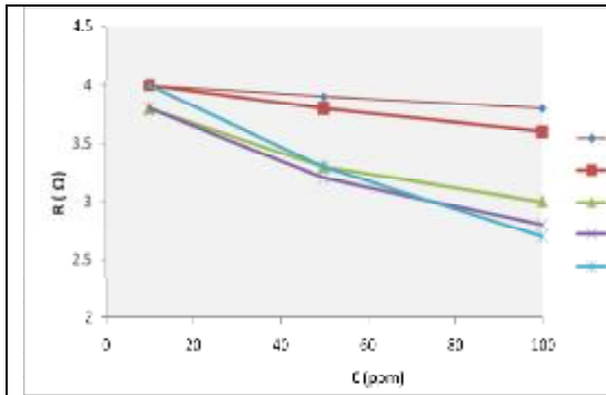
Figure (5) Resistance of ZnO thin film to H 2 S gas .
