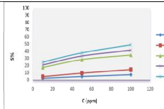
Figure (6) Sensitivity of ZnO thin film to H 2 S gas.
