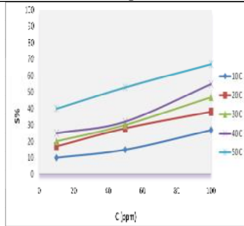
Figure (8) Sensitivity of ZnO thin film to NO 2 gas.
