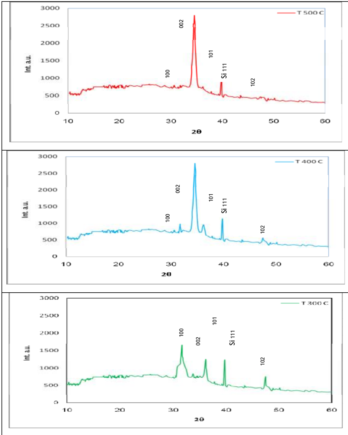
Figure (4) XRD result of ZnO thin film at 0.1 M
