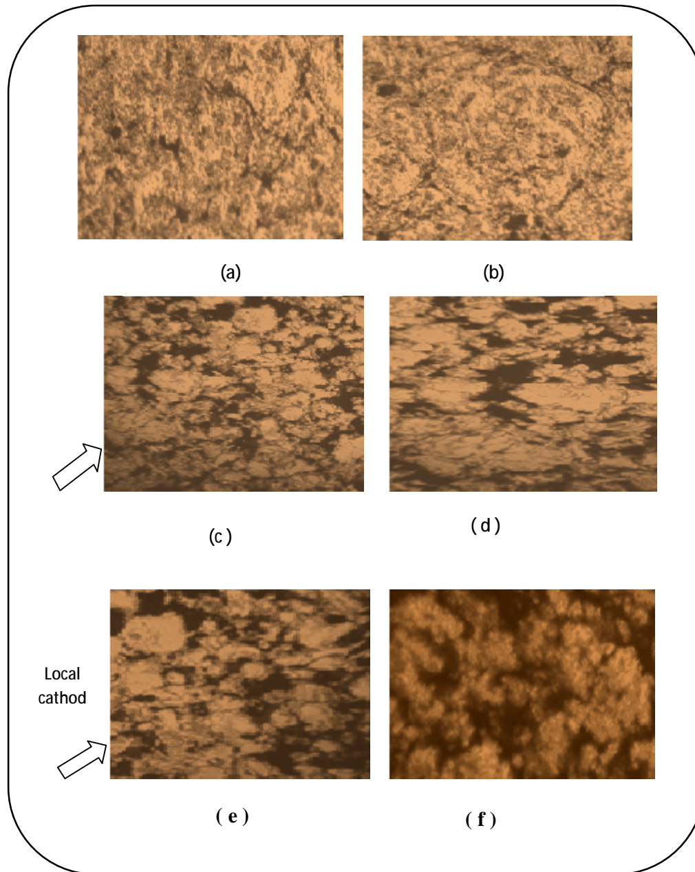
Figure. 18 Optical microscopic images (X100) show alumina particles after corrosion in 3.5% NaCl at different weight percent of Al 2 O 3 particulates in Al- matrix, a) 0% wt b) 5% wt c) 10% wt d) 15% wt e) 20% wt f) 25% wt
